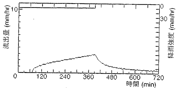
図3-7 CASE.4のR, Q
